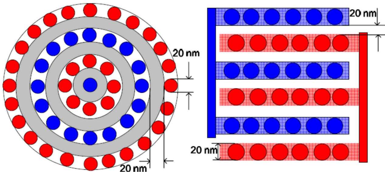
Two feasible vertical carbon nanotube capacitor structures—red and blue represent the anode and cathode, respectively.
